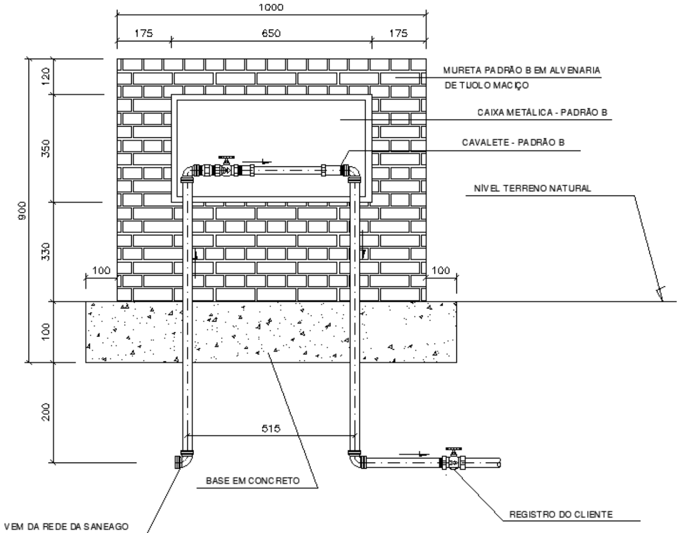
VISTA FRONTAL
