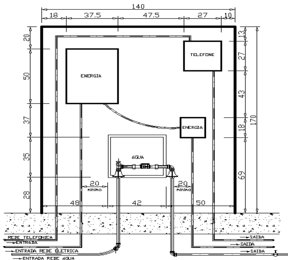
VISTA FRONTAL
